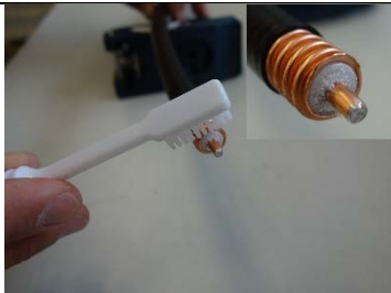
10) Clean up the inner conductor with brush and control the roundness of outer conductor
