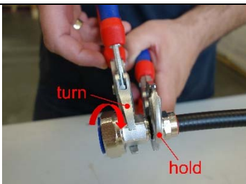
19) Use the wrenches as in the picture ( direction of rotation ).
