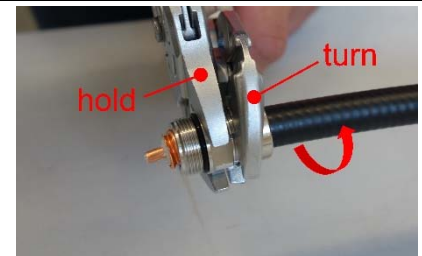
15) Use the wrenches as in the picture ( direction of rotation ).
