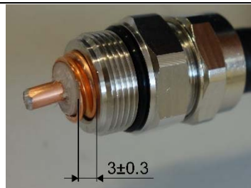
14) Slide back nut onto the cable until it is completely seated.
