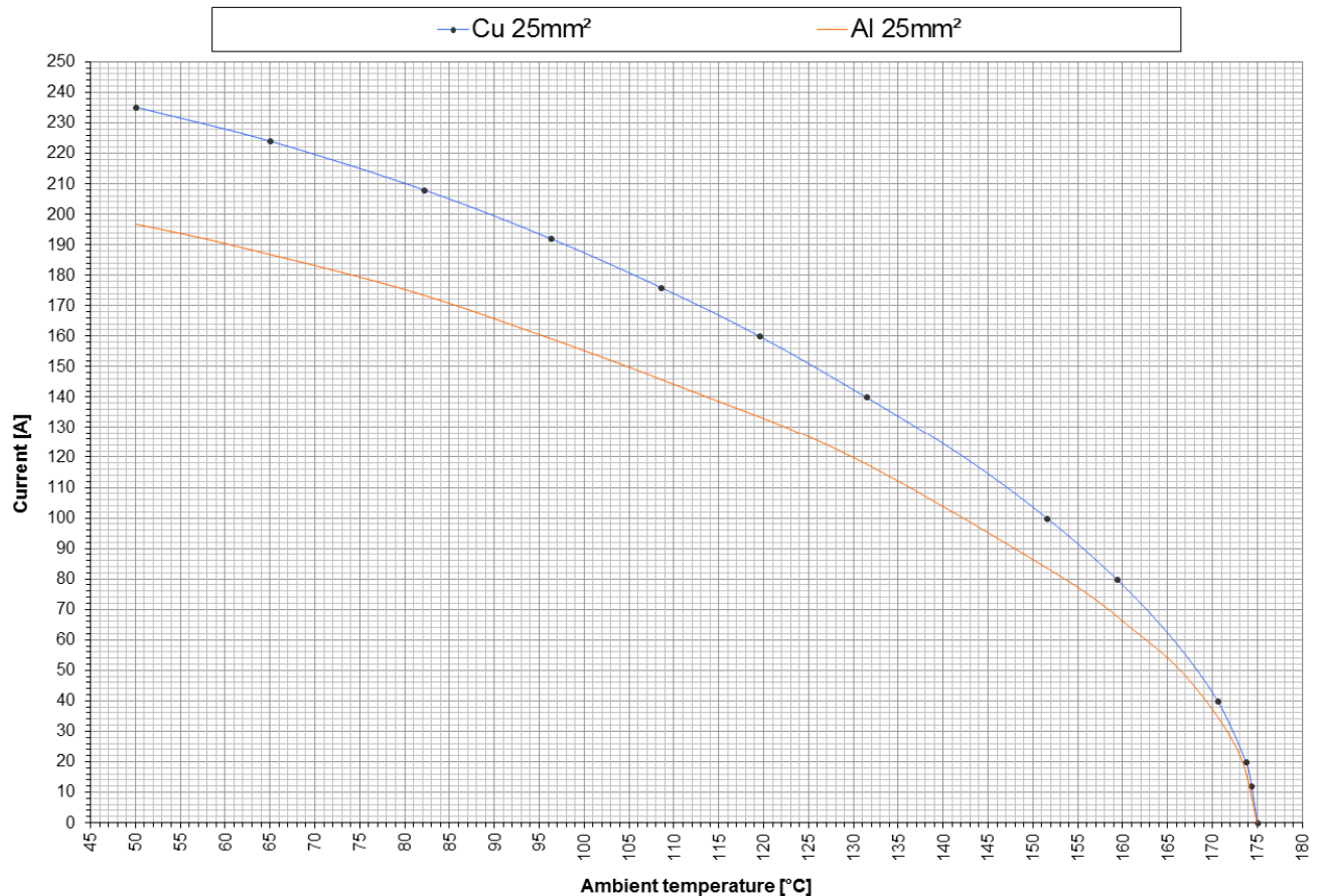
Copper & Aluminum cable 25mm 2 (80% Derating chart, free in air)
